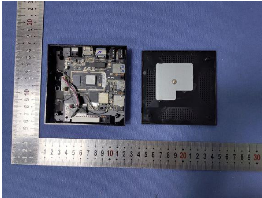
Fig.5 – Inside view
